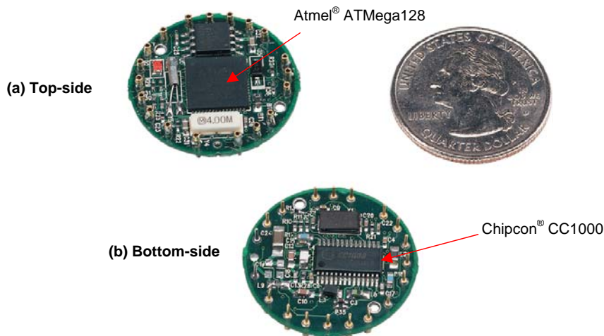
Figure 5-1. Photos of the MICA2DOT shown next to a US quarter: a) Top-side and b) Bottom-side. Typically the MICA2DOT has a 3 V coin-cell battery holder attached to the bottom-side, but it has been removed to show the details.
