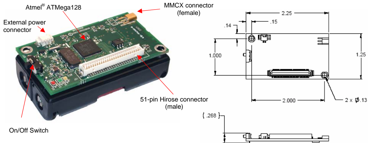
Figure 4-1. Left: Photo of a MICA2 (MPR4x0) without an antenna. Right: Top and plan views showing the dimensions and hole locations of the MICA2 PCB without the battery pack.
