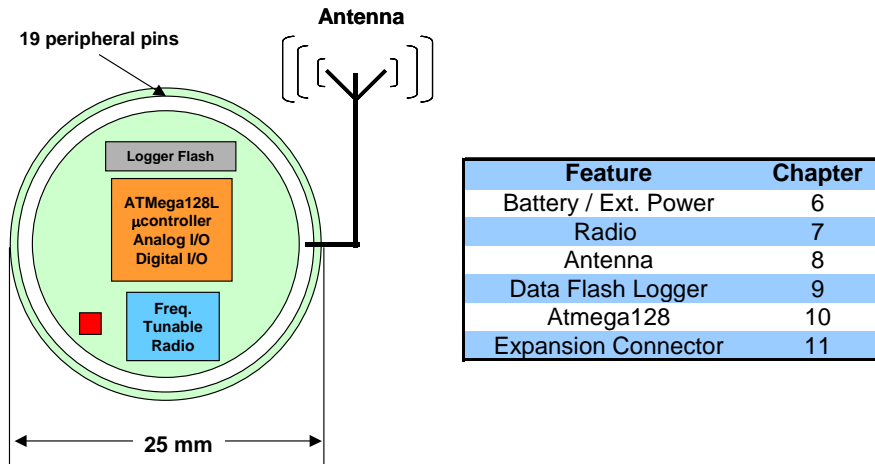
Figure 5-2. Block diagram of the MICA2DOT and listing of Chapters that discuss the components in greater detail.
