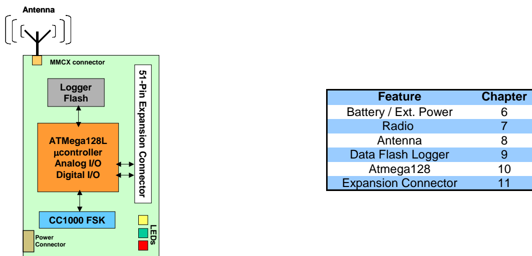
Figure 4-2. Block diagram of the MICA2 and listing of Chapters that discuss the components in greater detail.
