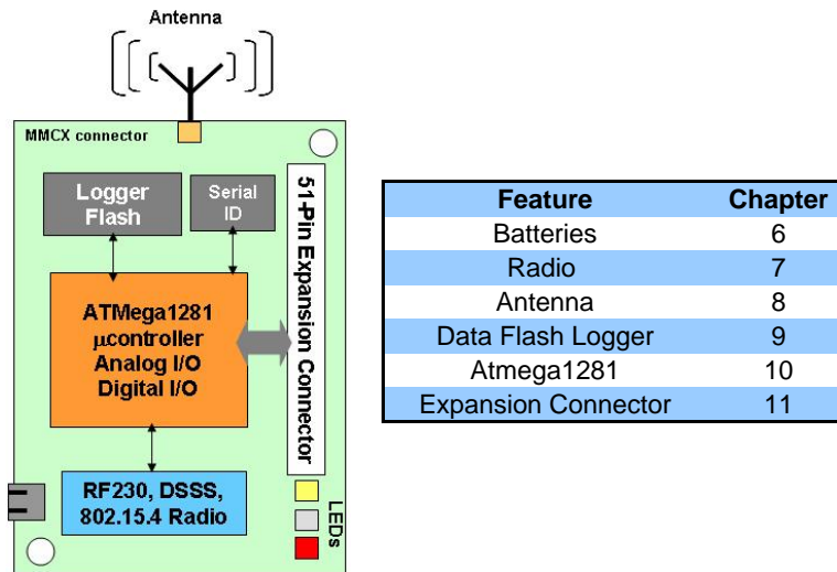
Figure 2-2. Block diagram of the IRIS and listing of Chapters that discuss the components in greater detail.
