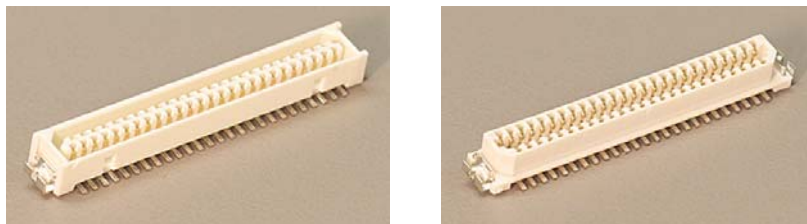
Figure 11-1. Hirose DF-51P-1V(54)—Digi-Key part no. H2175-ND—on left is used on the MICAz, MICA2, and MICA Motes boards. The Hirose DF9-51S-1V(54)—Digi-Key part no. H2163-ND—on right is the corresponding connector used on the MIB Interface Boards and Stargate Gateways.
