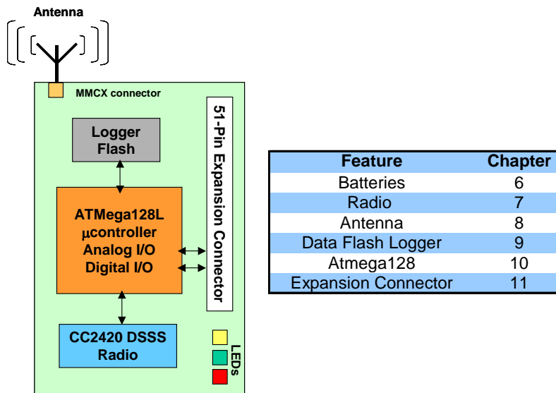
Figure 3-2. Block diagram of the MICAz and listing of Chapters that discuss the components in greater detail.
