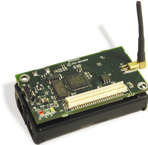
Figure 3-1. Photo of the MPR2400—MICAz with standard antenna.
